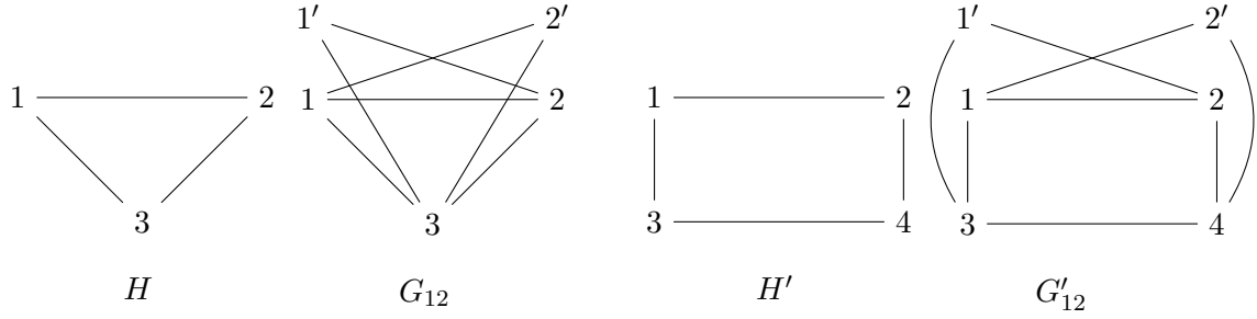
Figure 1: Two constraint graphs H and H' with corresponding supergraphs G_{12} and G'_{12} .
