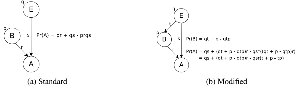
Figure 1: The Burglary Alarm Earthquake example.
