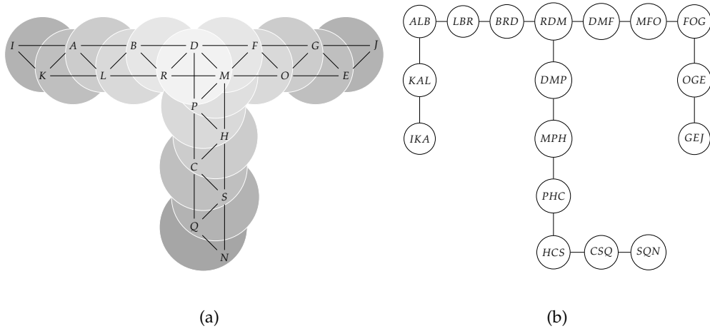
Figure 2 (a) An optimal tree decomposition of graph G in Figure 1; this is a set of overlapping clusters of G 's vertices, arranged in a tree. (b) The high-level treelike structure of G becomes apparent when it is drawn ignoring G 's edges.
