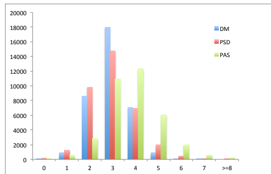
Figure 11 The distribution of relative treewidth for SemEval 2015 semantic dependency graphs.
