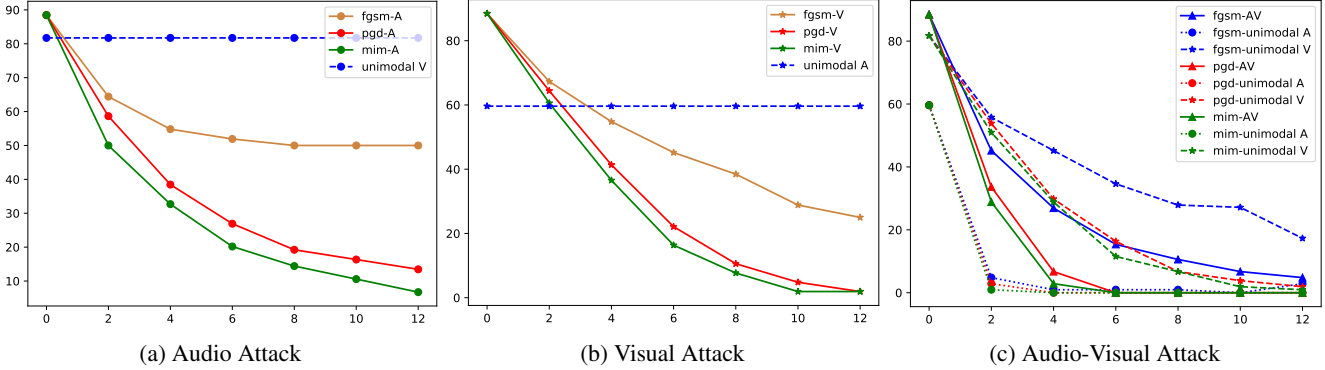
Figure 3: Adversarial robustness against multimodal attacks on the MIT-MUSIC. The x-axis denotes the attack strength ( \times 10^{-3} ) and we set \epsilon_a = \epsilon_v in the audio-visual attack for a better illustration. For the single-modality attack, the attacked audio-visual models in (a) and (b) still have clean visual and audio information, respectively. But, when adversarial perturbations become larger, joint perception models with one attacked modality become even worse than the corresponding individual perception models. Thus, an unreliable modality could weaken perception by the other modality in audio-visual models. A similar observation can also be found in the audio-visual attack (e.g., -AV vs. -unimodal V).
