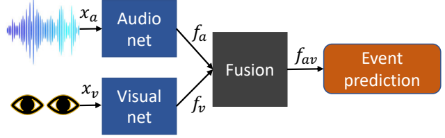
Figure 2: Audio-visual event recognition network. It integrates audio and visual content to predict the event category. To address the problem, we introduce an audio-visual network 2 as shown in Fig. 2, which can integrate information from the both modalities to infer event labels. It uses an 1D convolution-based audio network to extract an audio feature: f_a \in \mathcal{R}^d from x_a . ResNet [33] is adopted as the visual network to extract a visual feature f_v \in \mathcal{R}^d from x_v . The audio and visual features are integrated by a fusion function outputting a fused feature: f_{av} . In practice, we obtain f_{av} = [f_a; f_v] via concatenating the audio and visual features. Taking the f_{av} as an input, a fully-connected layer with a softmax is used to predict its event class probability p . The cross-entropy objective function: \mathcal{L}_{CE} = -\sum_{i=1}^k y_i \log(p_i) , where k is the category number, is used to force the model to learn discriminative features for each class that be mapped to correct output space.
