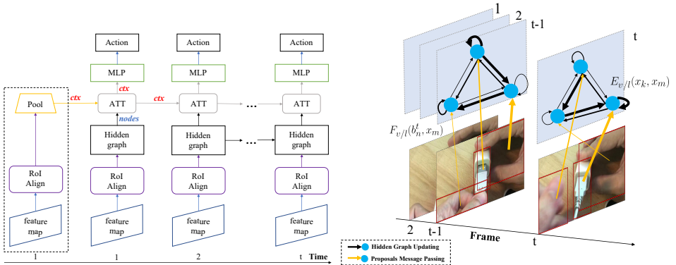
(a) The unrolled version of our graph network (backbone ConvNet and RPN are omitted). (b) The graph building process at each time step t-1 and t .
