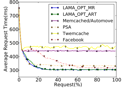
Figure 4: Average response time from cold-start to steady state
