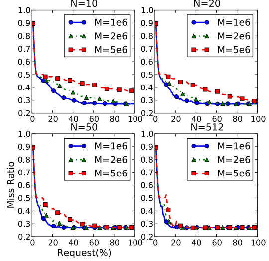
Figure 8: Different combinations of the repartitioning interval M and the reassignment upperbound N
