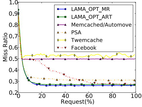
Figure 3: Facebook ETC miss ratio from cold-start to steady state
