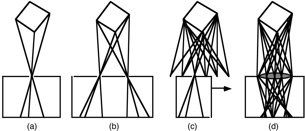
Fig. 1. Diagram from Leonardo's notebooks illustrating the fact that the light rays leaving an object's surface may be considered to form a collection of cones (which Leonardo calls “pyramids”), each cone constituting an image that would be seen by a pinhole camera at a given location.
