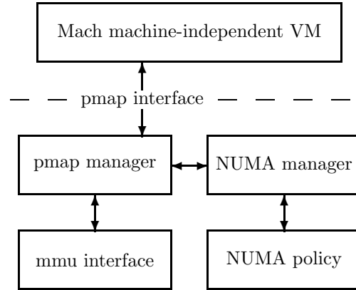
Figure 2: ACE pmap Layer
