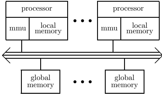
Figure 1: ACE Memory Architecture
