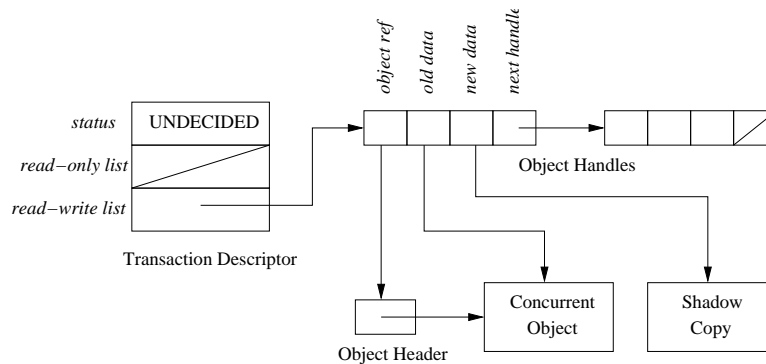
Fig. 2. The basic Transactional Memory Structure in FSTM
