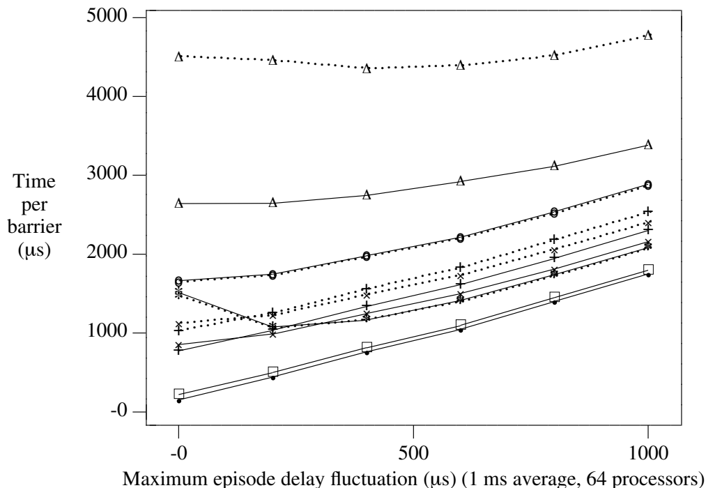
Figure 10: Dependence of performance on skew in process arrival times (Butterfly 1).
