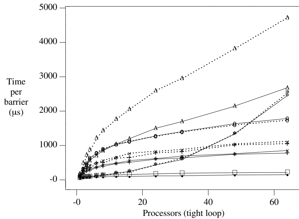
Figure 8: Basic barrier performance (Butterfly 1).
