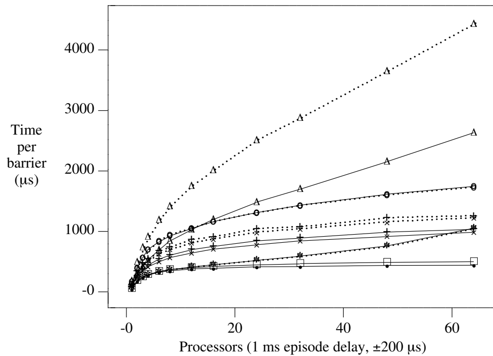
Figure 9: Barrier performance given time for computation (Butterfly 1).
