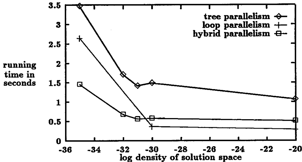
Figure 3: Performance of the three approaches over varying solution space densities.
