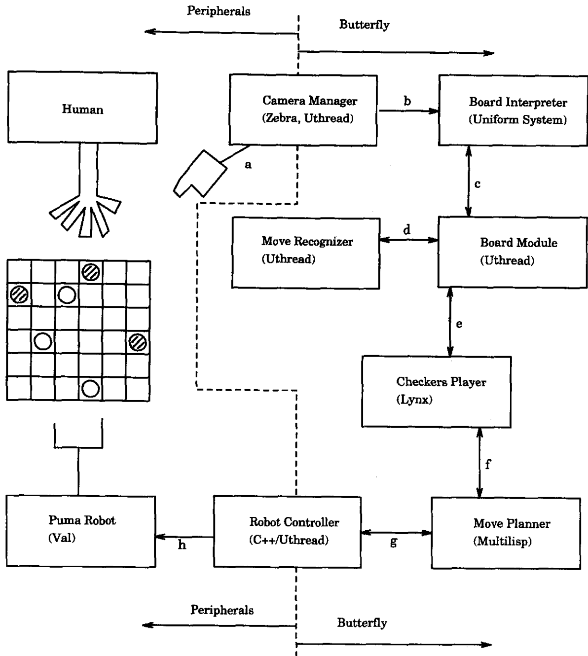
Figure 1 Functional modules and communication paths in the Checkers Player. Multiple models of parallelism (to the right of the dotted line) are implemented under Psyche on the Butterfly. Perceptual and motor modules (to the left of the dotted line) reside on the Butterfly and in peripherals.
