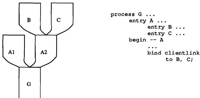
Figure 2: A cactus stack
