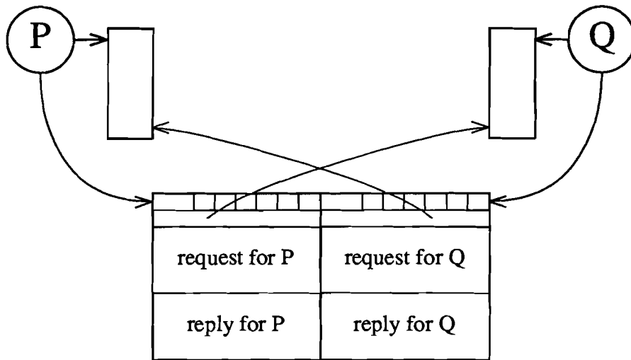
Figure 5: Chrysalis link implementation
