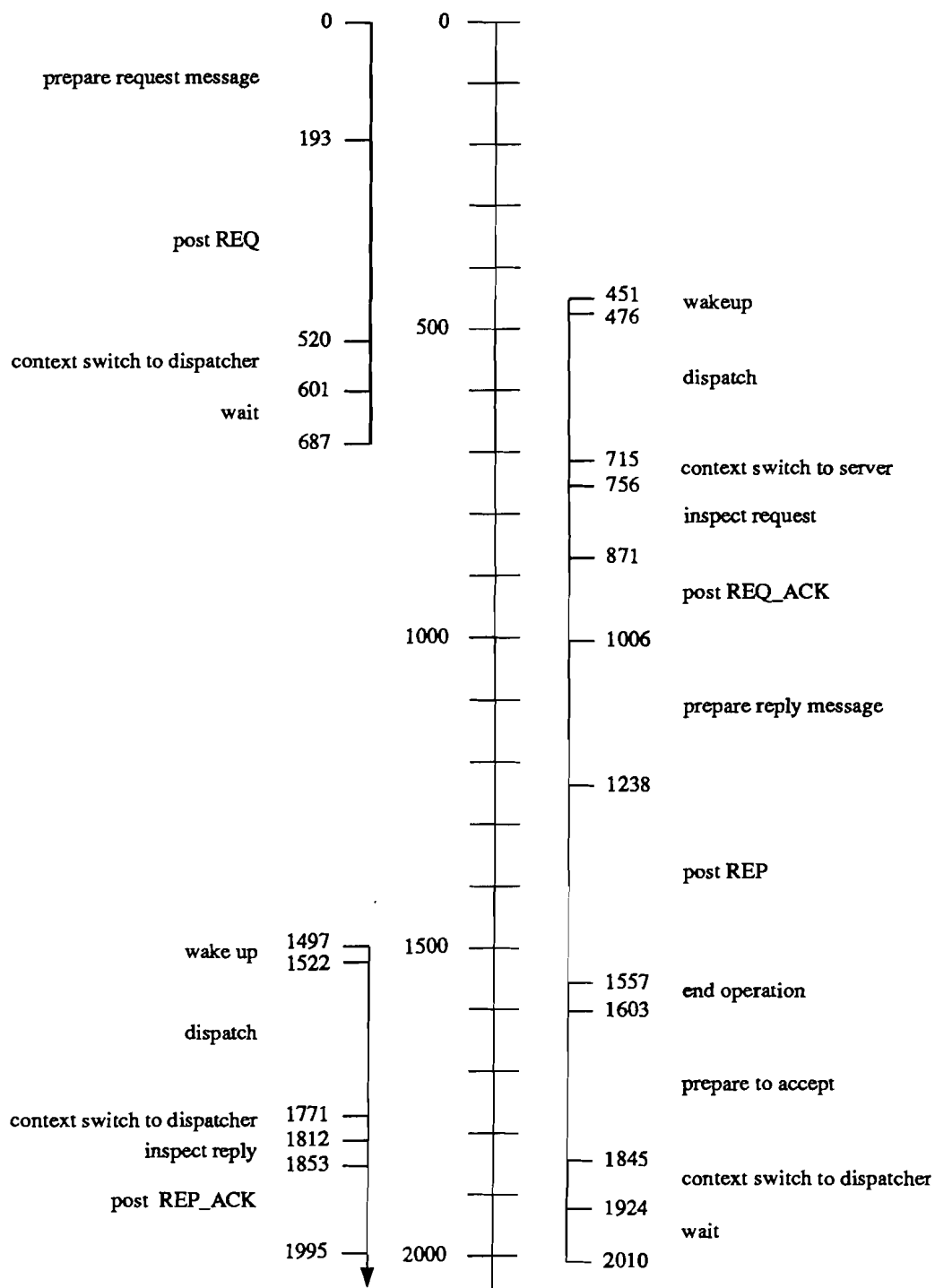
Figure 7: Timeline for a simple remote invocation
