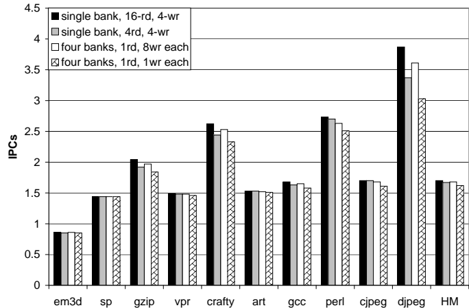
Figure 5. IPCs for the conventional and the base case (single bank with four read and four write ports), and for organizations with four banks. The third bar shows the effect of limited read ports, the fourth shows the effect of limited read and write ports.
