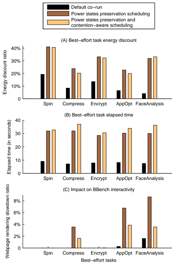
Figure 2: Experimental results of running interactive application Bbench web browsing with various best-effort tasks under different scheduling strategies. We show the best-effort task energy discount (A), best-effort task elapsed time (B), and impact on Bbench’s interactivity (webpage rendering slowdown) (C).
